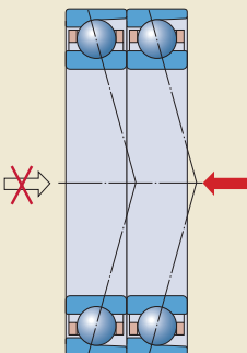
Tandem arrangement
