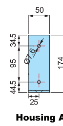
▲ Housing (U-shape) - ST 095ES
