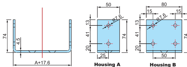
▲ Housing (U-shape) -ST 044S
